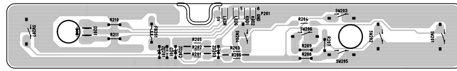
2. CONTROL BOARD (Solder Side)
